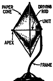
Early cone loudspeaker.
